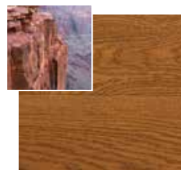
GRAND CANYON
