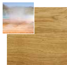
YELLOWSTONE
