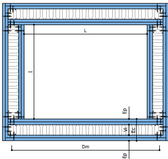
Gaine technique verticale 4 faces – coupe horizontale
