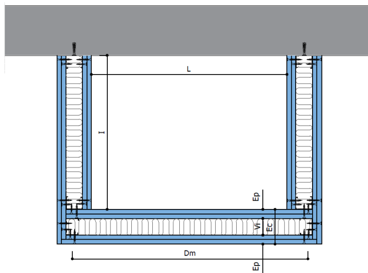
Gaine technique verticale 3 faces – coupe horizontale
