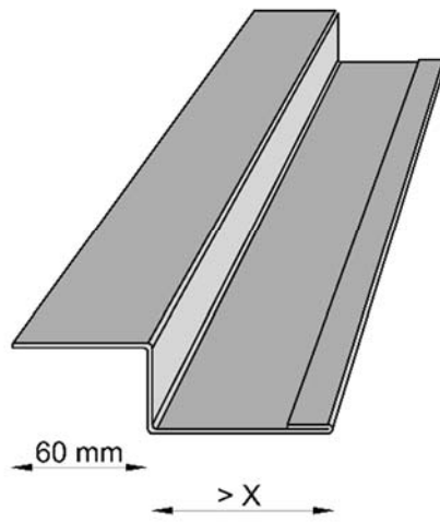
Figure A4 - Joint de dilatation
