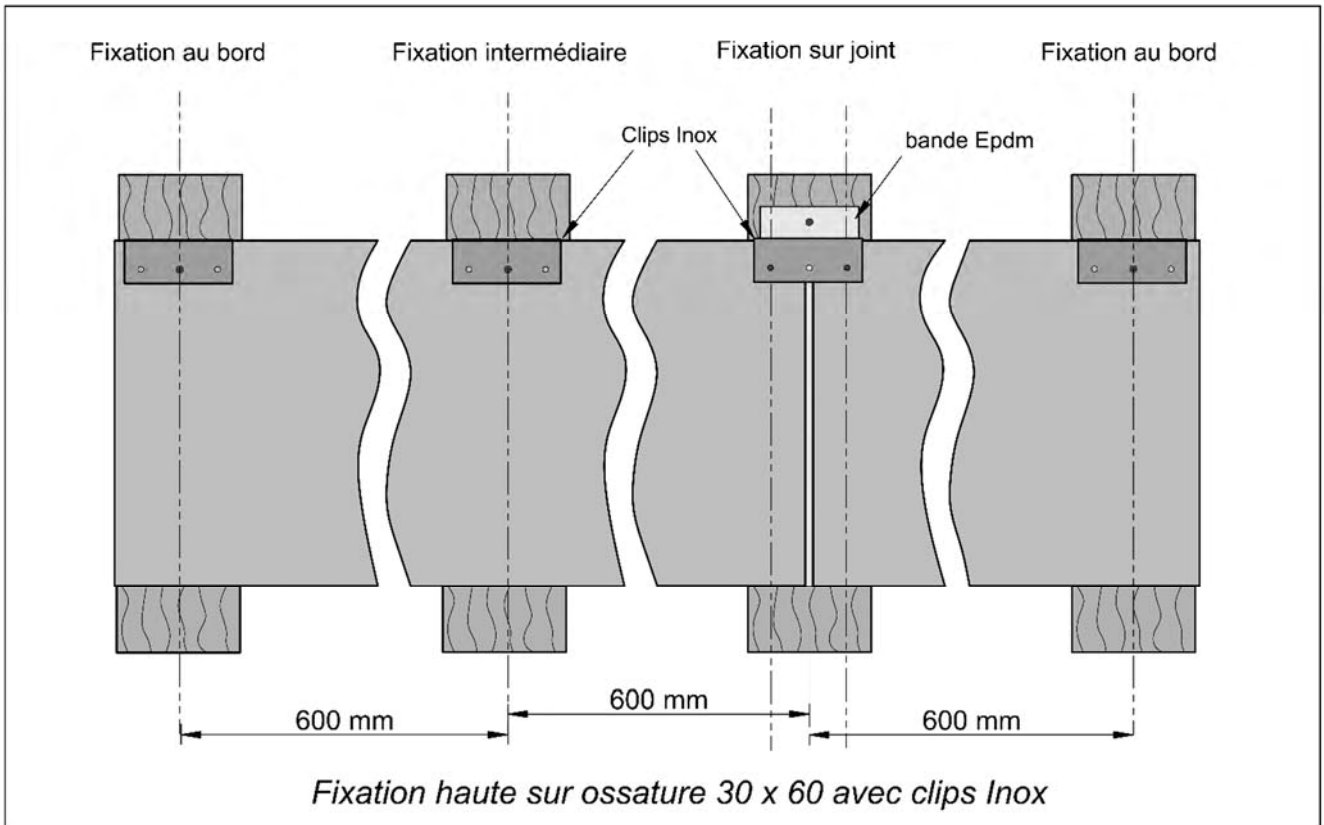
Figure 3.1 - Fixations des clins
