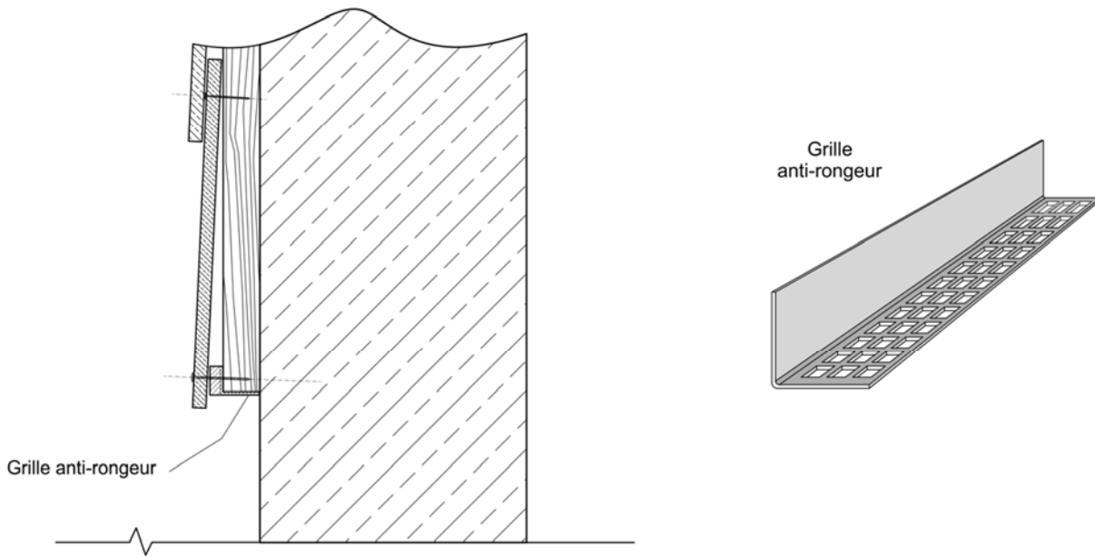
Figure 12 – Grille anti-rongeur
