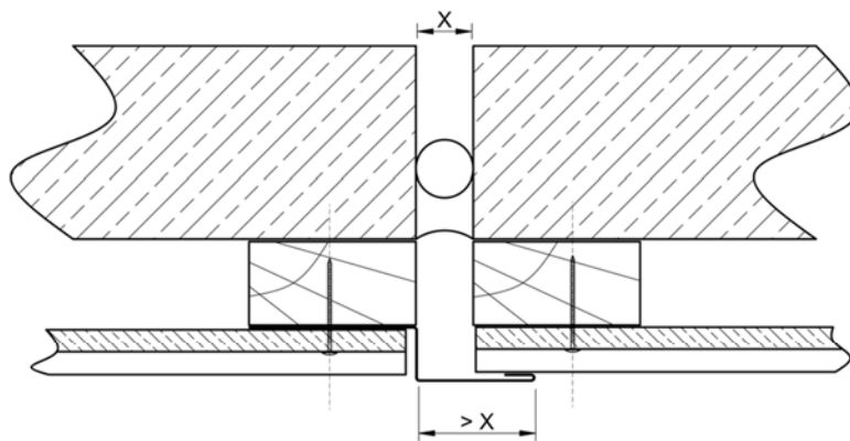
Figure 12 – Grille anti-rongeur
