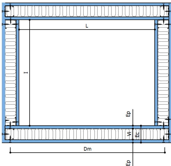
Gaine technique verticale 4 faces – coupe horizontale
